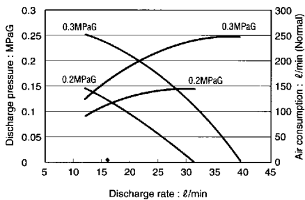
Performance Curves for PS-E 40H (at 20°C)
