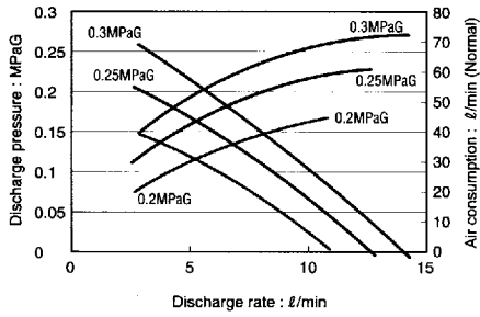
Performance Curves for PS-E 10H (at 20°C)
