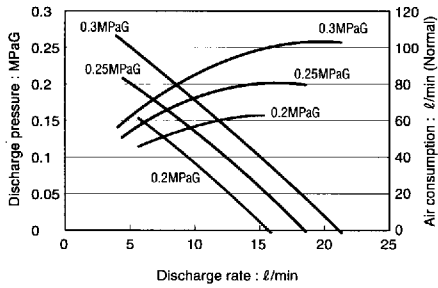
Performance Curves for PS-E 20H (at 20°C)
